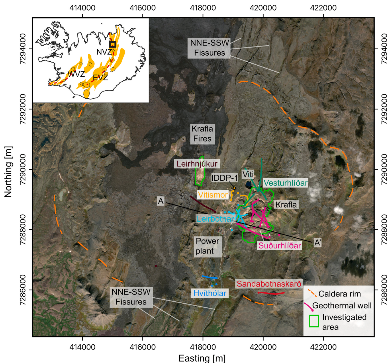
Fig. 1. Location of the Krafla geothermal field. The geothermal system developed in the 8–10 km-width caldera of Krafla (orange line), and is divided into 5 subfields: Leirbotnar (Vitimor included), Suðurhlíðar, Vesturhlíðar, Hvíthólar, and Sandabotnaskarð (Árnason, 2020; Scott et al., 2022). Soil CO 2 flux measurements were carried out over both the main production area of the geothermal field (Suðurhlíðar, Vesturhlíðar, and part of Leirbotnar) and Leirhnjúkur (green perimeter). The circles and lines reflect the geothermal well heads and subsurface paths (from Mortensen et al., 2015). The inset (modified after Árnason, 2020) shows the location of Krafla in the Northern Volcanic Zone (NVZ) of Iceland. WVZ and EVZ stands for Western and Eastern Volcanic Zone, respectively. The yellow areas reflect fissure swarms and the black contours are the main central volcanoes. Red dashed lines display spreading zones. Background is from ESRI imagery. Coordinates refer to the WGS 84/UTM zone 28 N. (For interpretation of the references to colour in this figure legend, the reader is referred to the web version of this article.)
